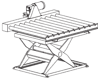
G-645 Scissor Lift with Chain Driven Live Rollers
