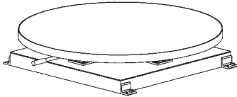
G-605 Manual Turntable with Detent Stop
