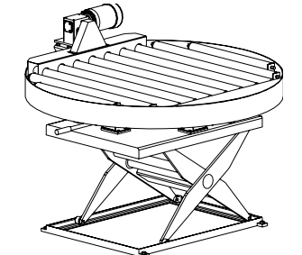
G-658 Scissor Lift with Manual Turntable and Power Rollers
