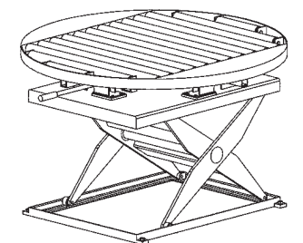
G-657 Scissor Lift with Turntable and Gravity Rollers
