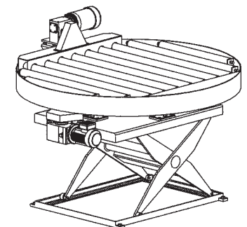
G-685 Scissor Lift with Power Turntable and Chain Driven Live Rollers
