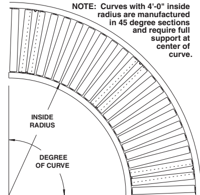
Double roller design
