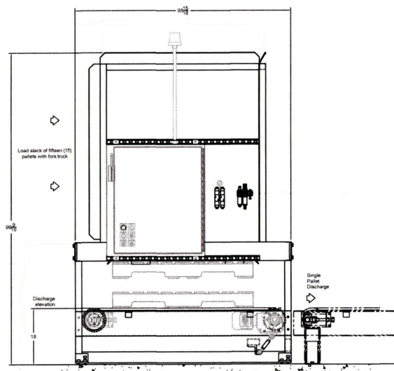
Automatic Pallet Dispenser Model 50-57
