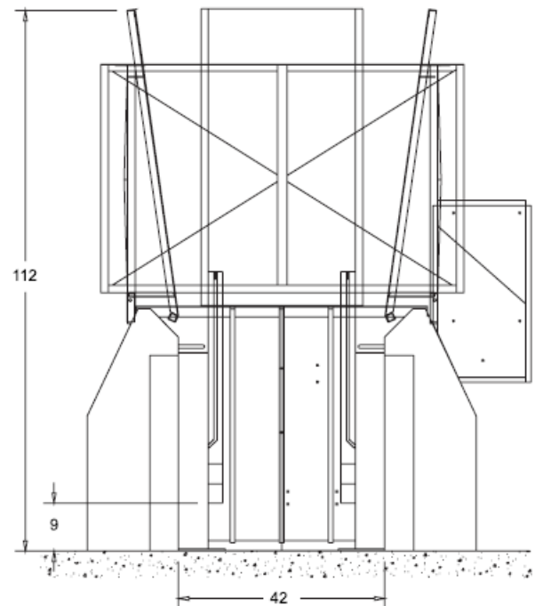
Typical Machine Configuration
