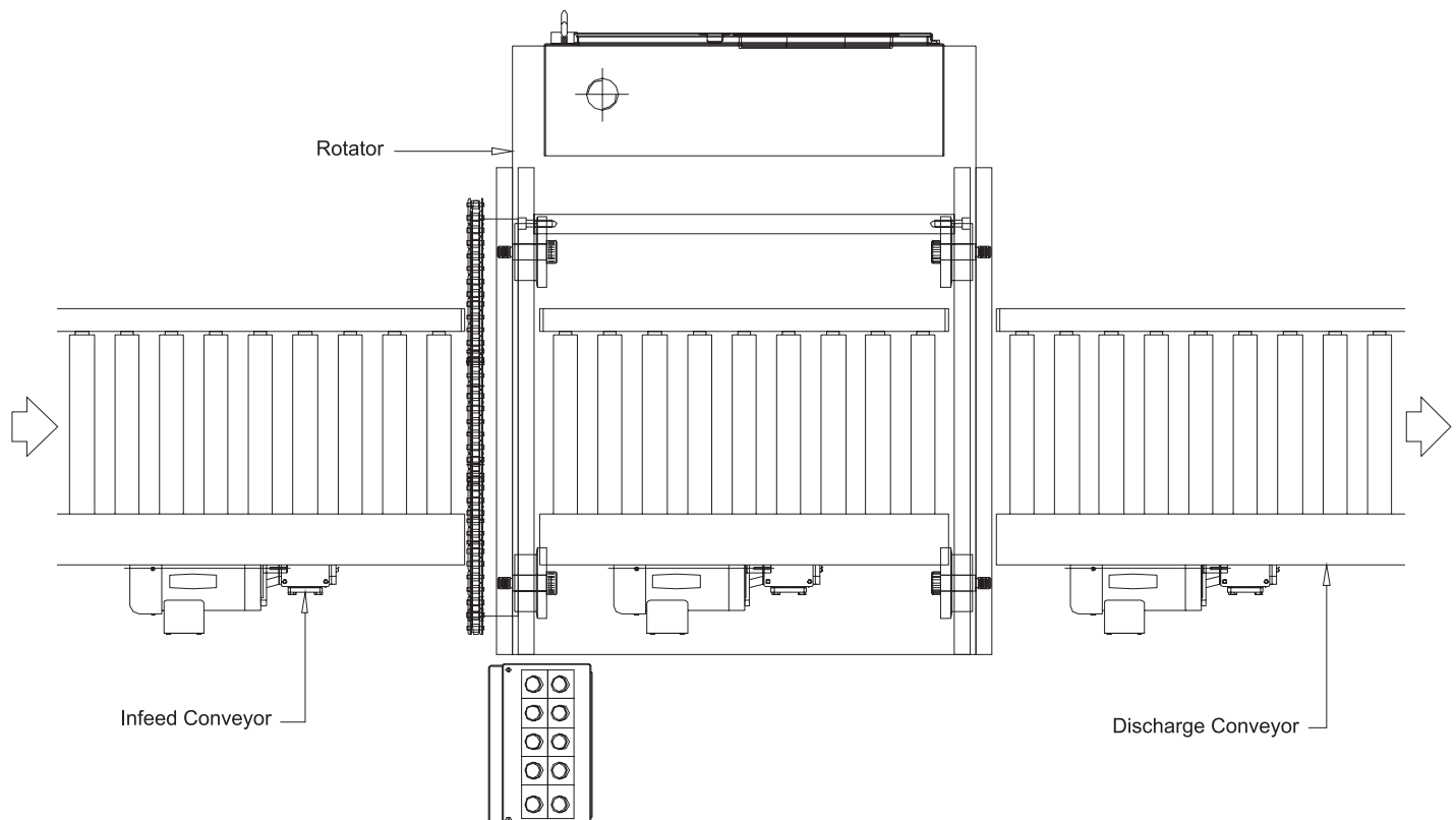
DL-3500 Barrel Type Inverter
