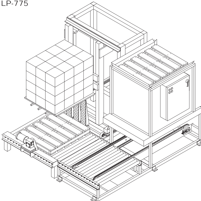
LP-775 Load Transfer System with Lifting Tines
