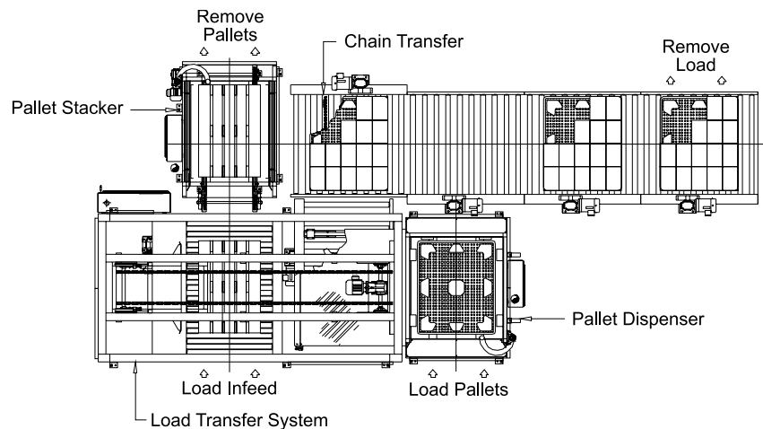
RM-1150 Pallet to Pallet Load Transfer System "Z" Configuration
