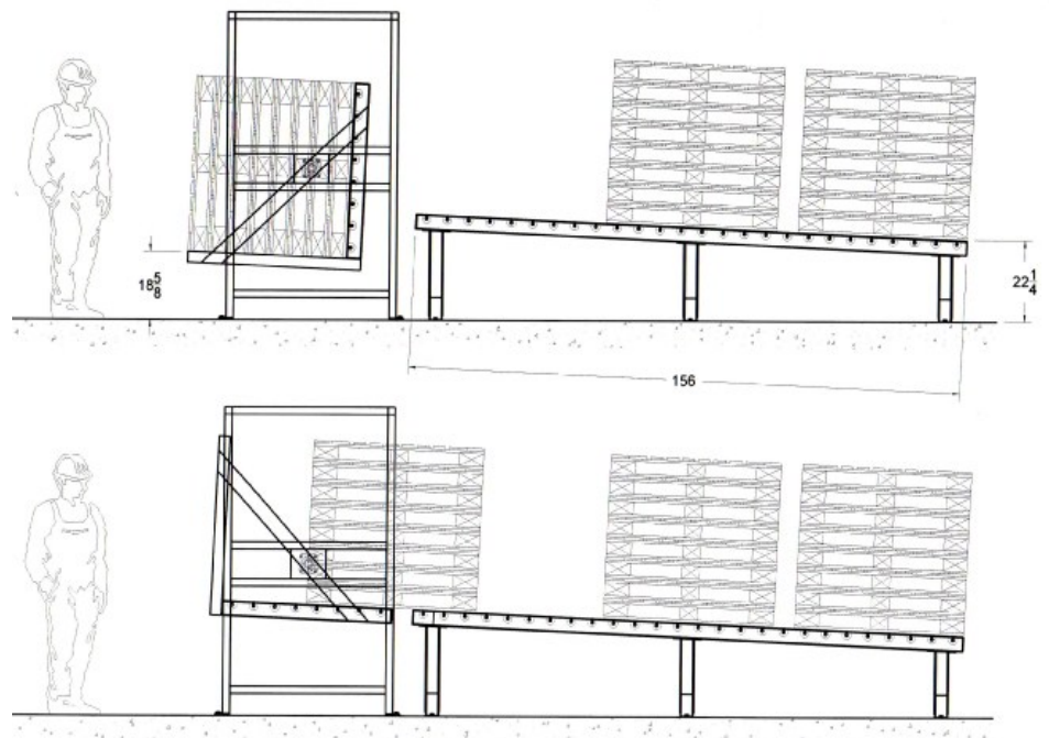
40-57 Manual Pallet Stacker
