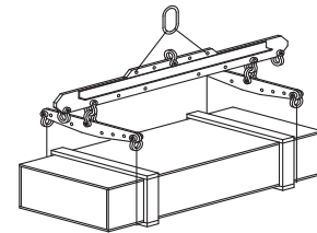
CUSTOM 4 POINT LIFT
