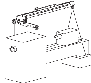
CUSTOM 3 POINT LIFT
