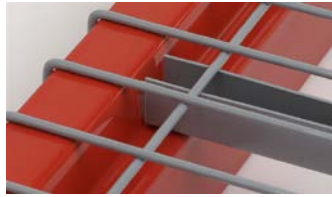
Standard U-Channel
