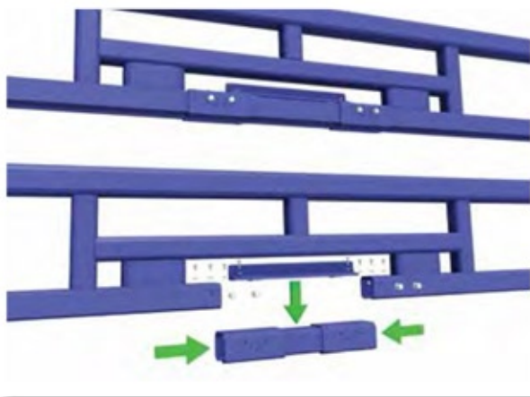
Maintenance Gates
