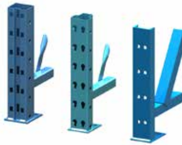
Rack Profiles
