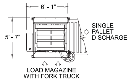
Automatic Pallet Dispenser Model 50-57 with Magazine Extension
