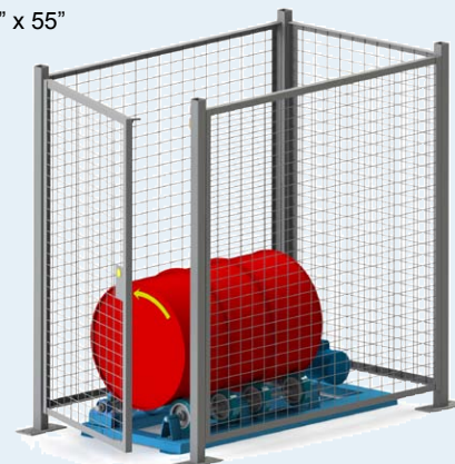
Guard Enclosure with safety interlock model GEK-1-5154-1 shown with Drum Roller (sold separately)
