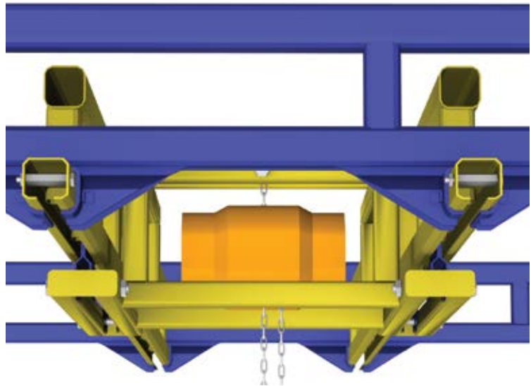
Nested Trolley
